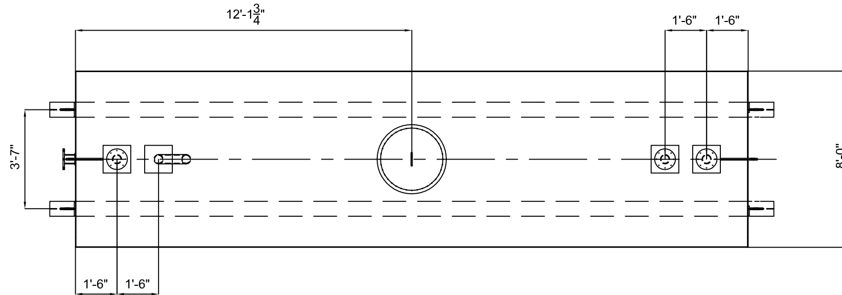
TOP VIEW
