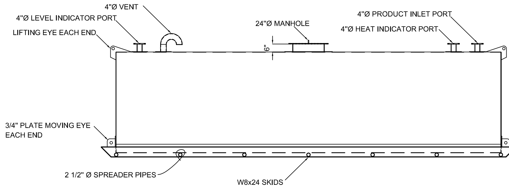
FRONT VIEW
